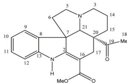
Minovincine (4)
